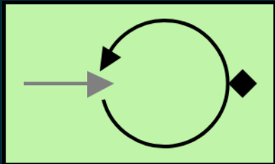
Polling Consumer
