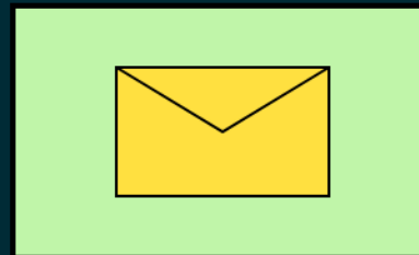
Envelope Wrapper
