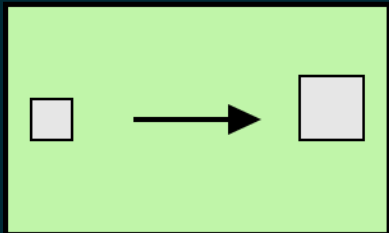
Content Enricher
