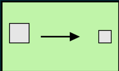
Content Filter
