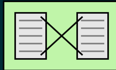
Message Translator
